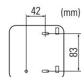
Vista posteriore Rear view
